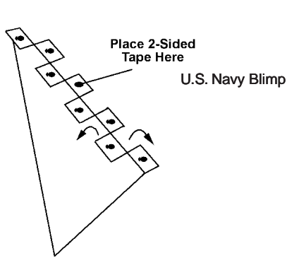
Diagram #3 - Alternate bending tabs left, then right / Applying 2-Sided tape to folded Rudder Fin Tabs.
