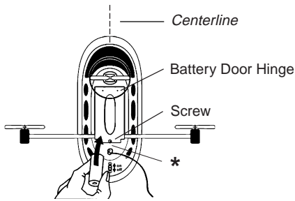
Diagram #1 - Installing the CR123A Battery into the Thruster Engines Module. * Note where the Ballast Putty can be placed.
