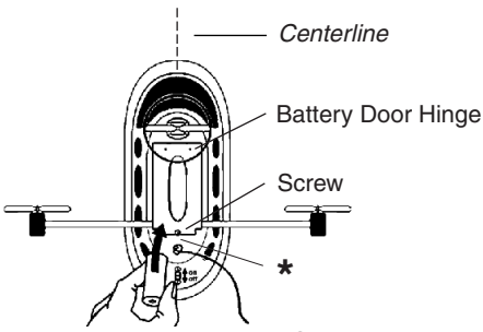
Diagram #1 - Installing the CR123A Battery into the Thruster Engines Module. * Note where the Ballast Putty can be placed.
