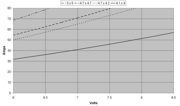
HA2825-5500 Current vs. Voltage with Propeller
