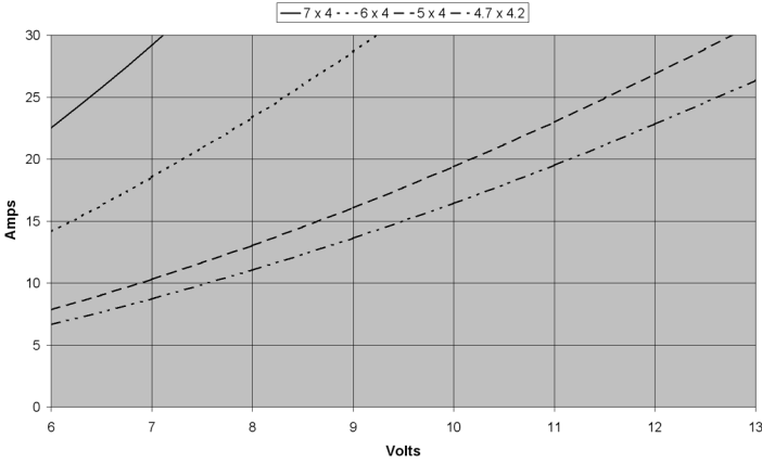
HA2825-3600 Current vs. Voltage with Propeller
