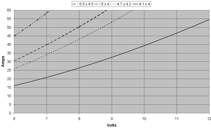
HA2825-4400 Current vs. Voltage with Propeller
