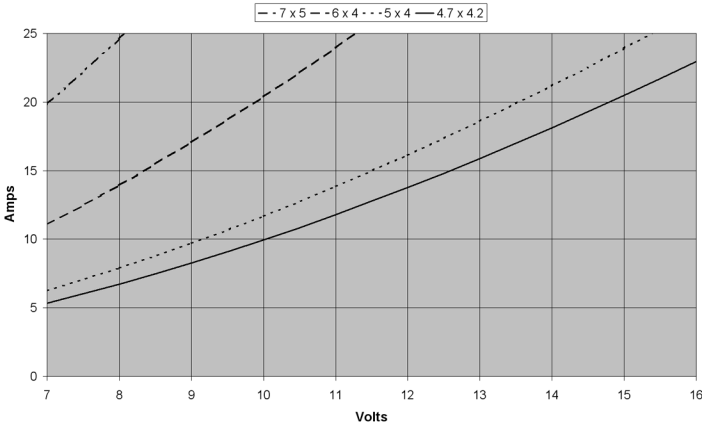
HA2825-2700 Current vs. Voltage with Propeller
